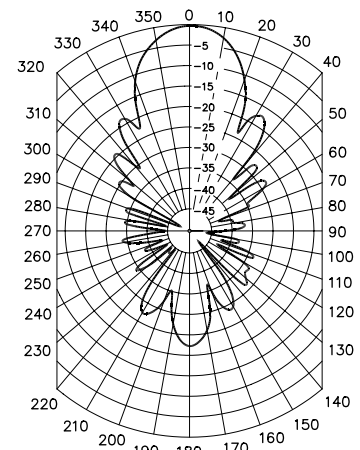
Fig 40—Measured E-plane pattern for the 22-element Yagi. Note: This antenna pattern is drawn on a linear dB grid, rather than on the standard ARRL log-periodic grid, to emphasize low sidelobes.
